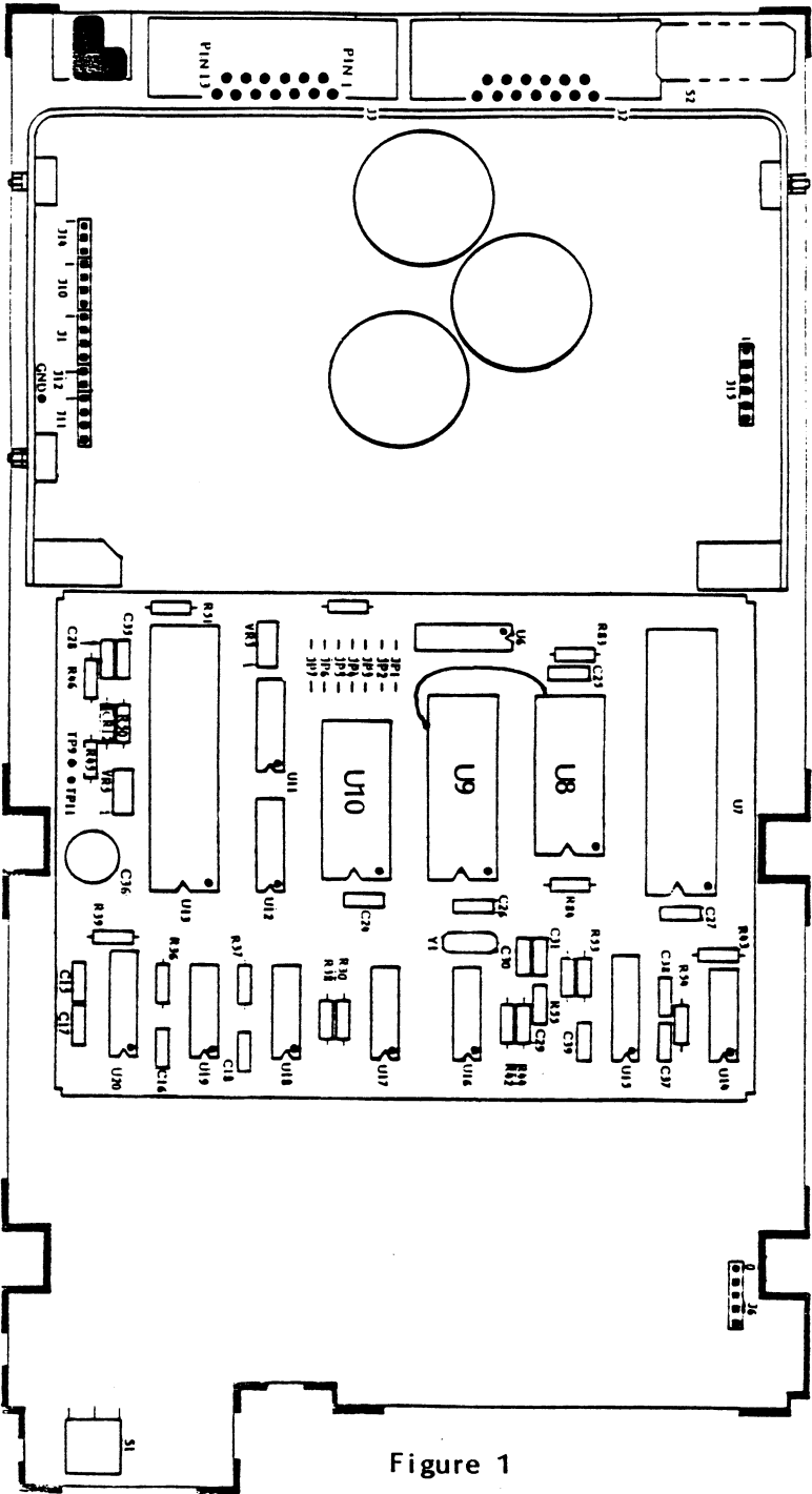
1050 P C B Layout
